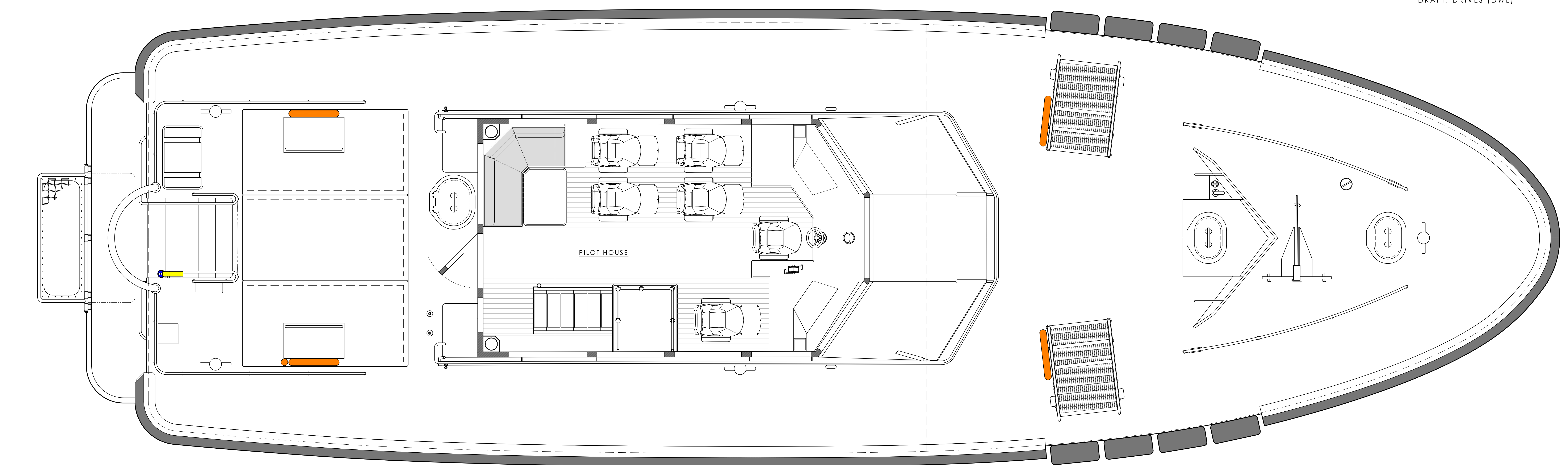
MAIN DECK PLAN
