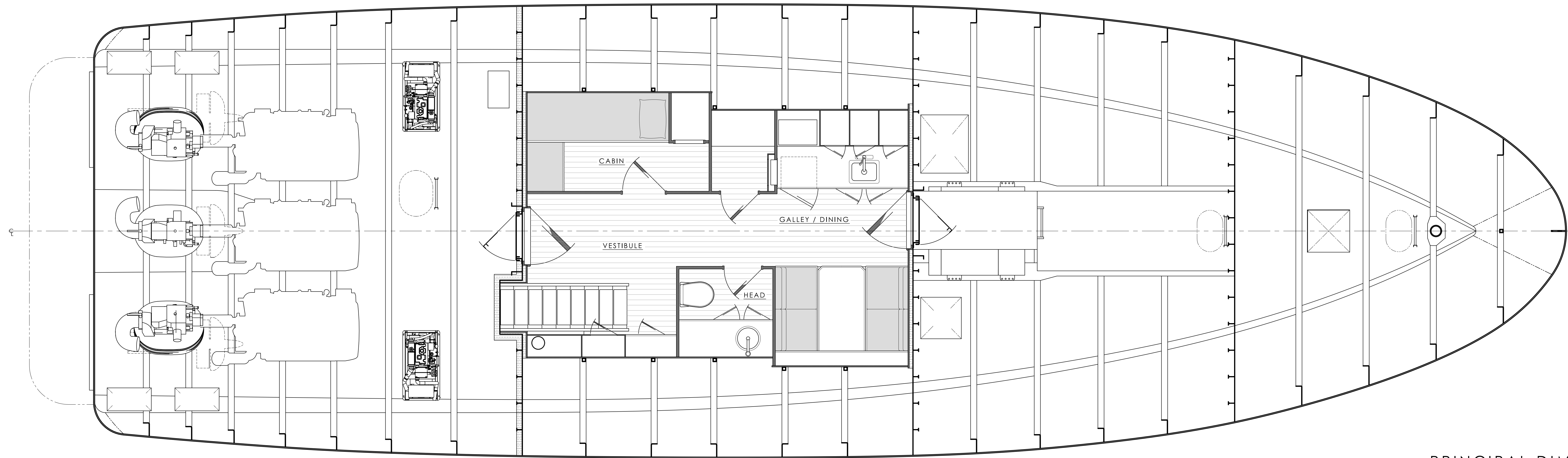
BELOW DECK PLAN
